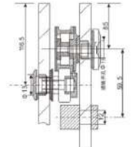
30x10 sectional installation of square pipe with jumping-proof pillar
